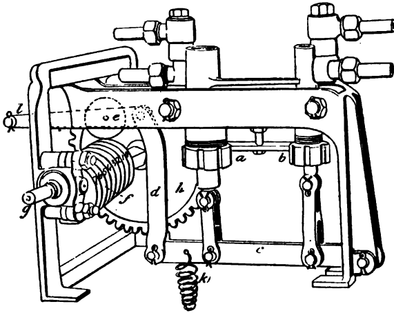
FIG. 105.—Serpollet's Fuel and Water Pumps. The water pump, a , and the fuel pump, b , are operated from the lever, c . This is given an up-and-down movement by the link, d , whose stroke is varied by the stepped cam, f , on which bears the roller, e , on the rod pivoted at i . The rotary movement of the cam shaft, g , is imparted by the spur wheel, h .
